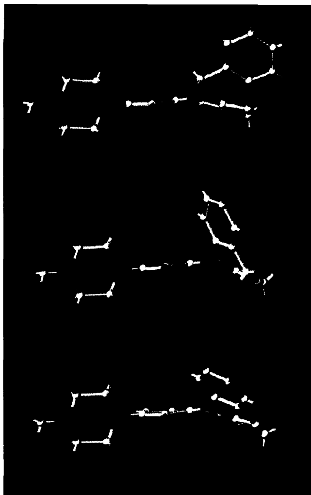
Figure 2. Modelled structures of tetracyclic quinolones 5a , 10a and 11 viewed from the N-1 to 4-keto direction.
