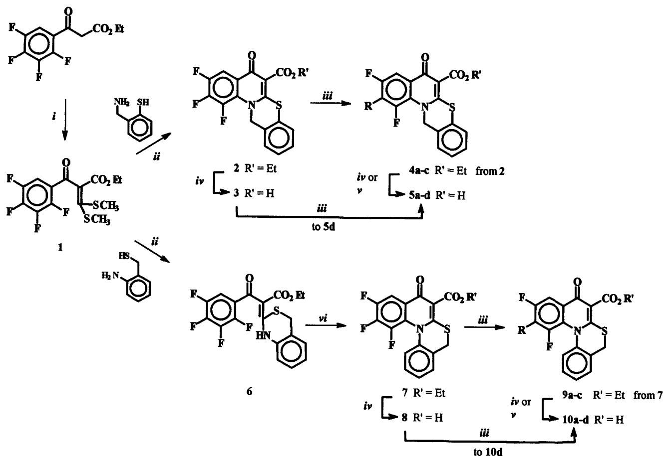
Scheme 1. Reagents: (i) DMSO/H 2 O, KOH, CS 2 , CH 3 I; (ii) Et 3 N, toluene, reflux; (iii) RH, Et 3 N, CH 3 CN, reflux; (iv) 18% HCl, EtOH, reflux; (v) 4% NaOH, EtOH, reflux; (vi) DBU, toluene, reflux.
